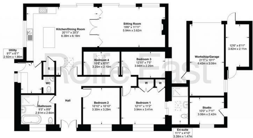
Floor Plan Approximate Floor Area 1,931 sq.ft (179.36 sq.m)
